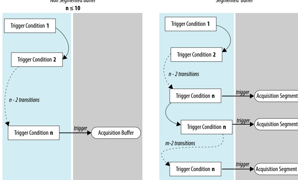
Figure 73. Sequential Triggering Flow
